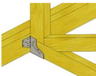
TM Hanger Used for fixing loose infill, mono & small std trusses to wallplate
