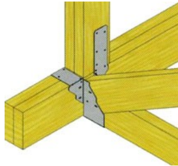
TS Truss Hanger Used for fixing single & girder trusses to girder trusses
