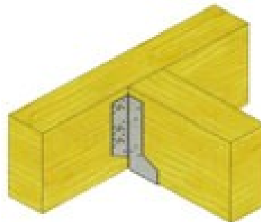
MHE Multi Hanger Used for fixing girder trusses to girder trusses
