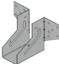
TM Hanger Used for fixing loose infill, mono & small std trusses to wallplate
