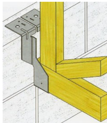
JH Masonry Joist Hangers Used for fixing trusses directly to brick or blockwork.
